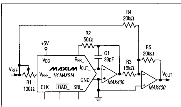
Figure 4. Bipolar Operation for 1/4 of MAX514
